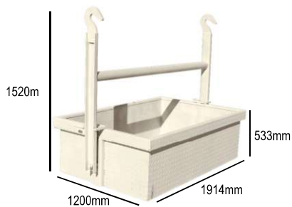
Box (1m3 Box with upper attachment) (CXC)
