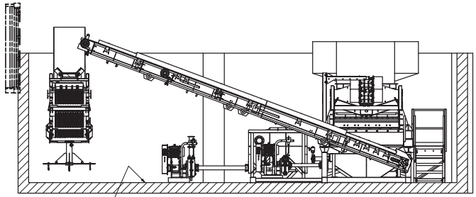
SECTION D-D ULTRA DRY ELEVATIONS SCALE 1" = 50'
