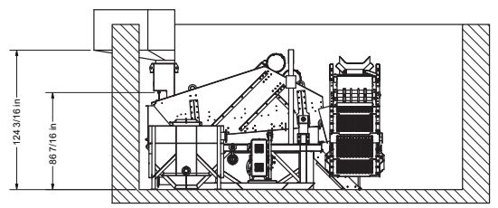
SECTION F-F SCALE 1" = 50'
