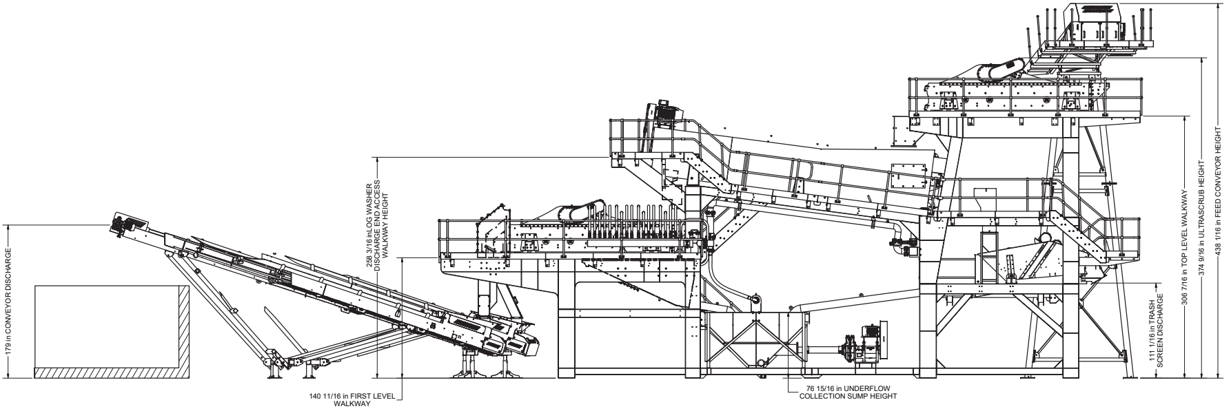
SECTION C-C ULTRASCUB ELEVATIONS SCALE 1" = 50'
